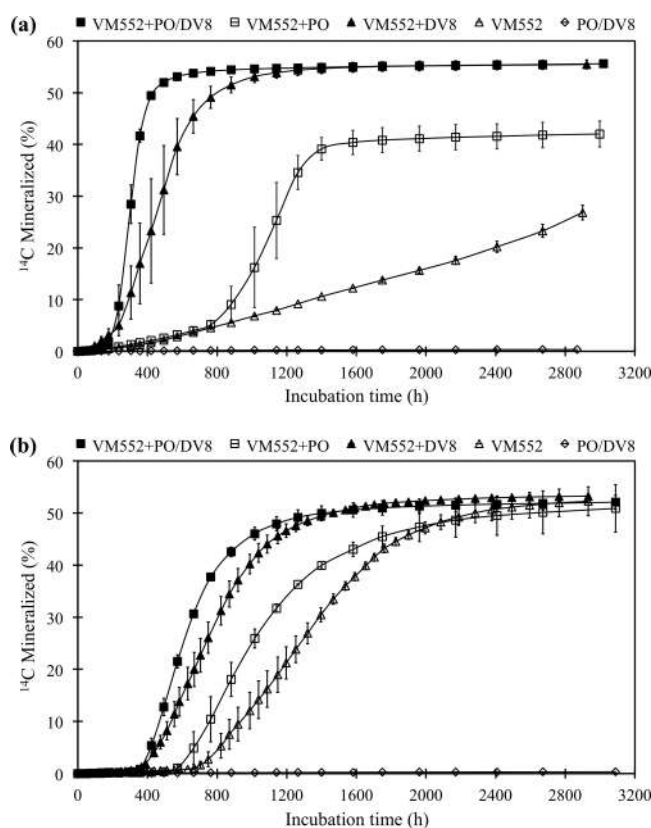
Figure 1. Effect of Pythium oligandrum mycelia on bacterial mineralization of ^{14}\text{C} -phenanthrene initially associated with the nonaqueous phase liquid (NAPL). The experiments were conducted under shaking (a) and static (b) conditions. The treatments included Mycobacterium gilvum VM552 plus P. oligandrum growing on DV8 agar (VM552+PO/DV8), M. gilvum VM552 plus P. oligandrum mycelia (VM552+PO), M. gilvum VM552 plus DV8 agar (VM552+DV8), M. gilvum VM552 alone as a positive control (VM552), and P. oligandrum growing on DV8 agar as a negative control (PO/DV8). Error bars represent the standard error from at least duplicate experiments.
