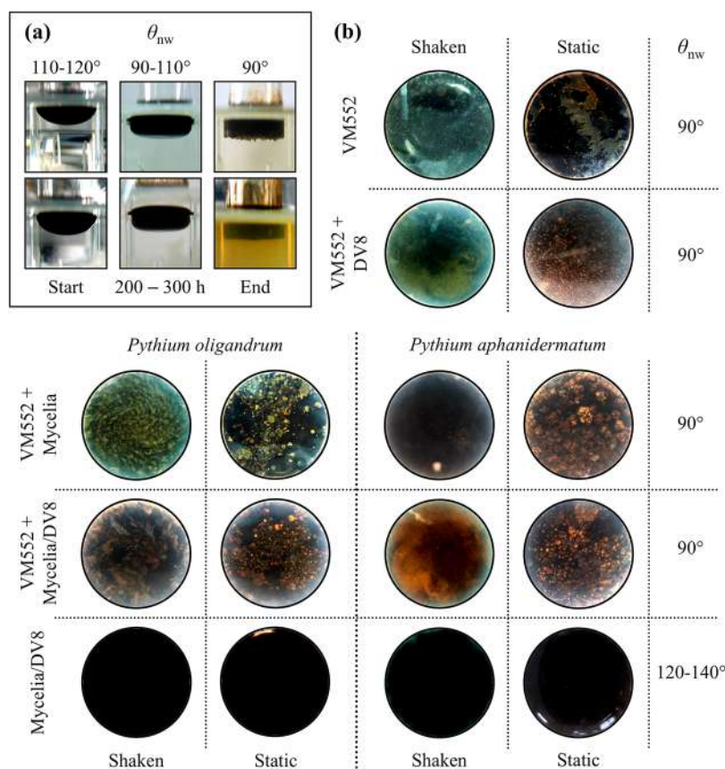
Figure 2. Effects of microbial growth on the morphological evolution of NAPL and macroscopic structures of microbial biofilms colonized at NAPL/water interfaces. The morphological evolution of NAPL determined with the change of contact angle ( \theta_{nw} ) was visualized along the mineralization experiments (a). The macroscopic structures of microbial colonization in form of biofilms at NAPL/water interfaces were photographed at the end of incubation (b). All photographs present in part a were derived from the experiments under shaken (top) and static (bottom) conditions that contained Mycobacterium gilvum VM552 and Pythium oligandrum growing on diluted V8 (DV8) agar. The photographs present in part b refer to all treatments indicated in Figure 1 and SI Figure S1. The diameters of these photographs correspond to the inner diameters of the glass cylinders (2 cm).
